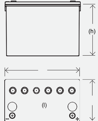
S12V4500PP S12V5200PP
